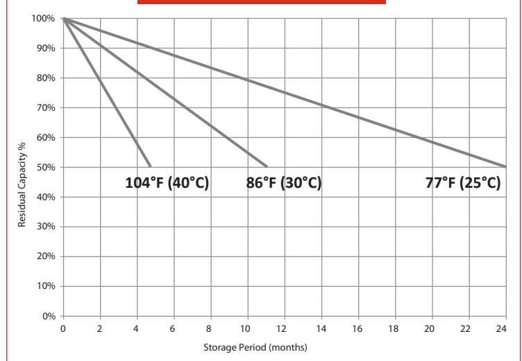
Self Discharge During Storage
