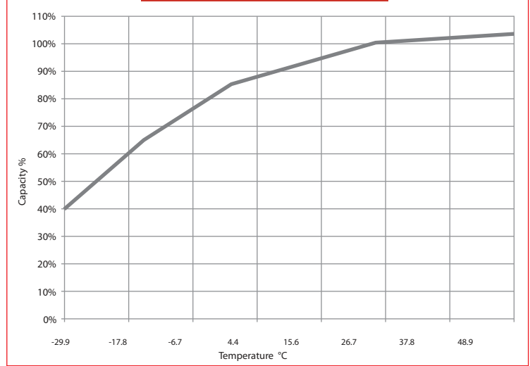
Temperature Versus Capacity
