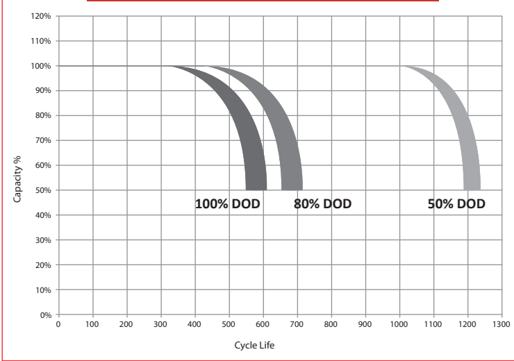
Depth of Discharge (DOD) Versus Cycle Life
