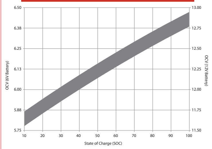
Open Circuit Voltage (OCV) Versus State of Charge (SOC)
